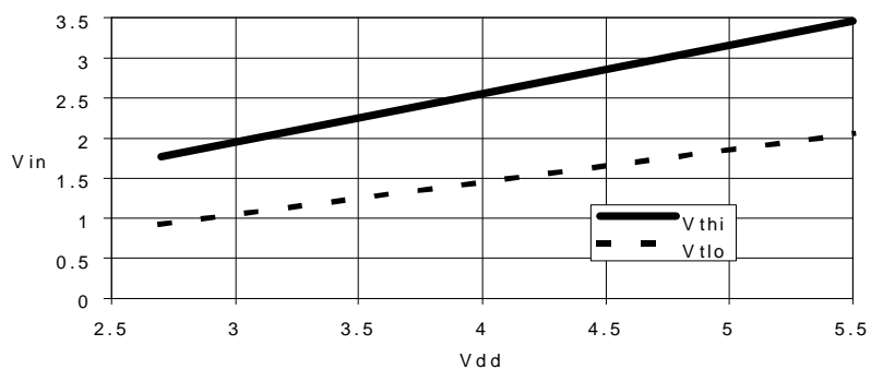
Figure 8 Typical Schmitt Trigger Input Voltage vs. V DD
