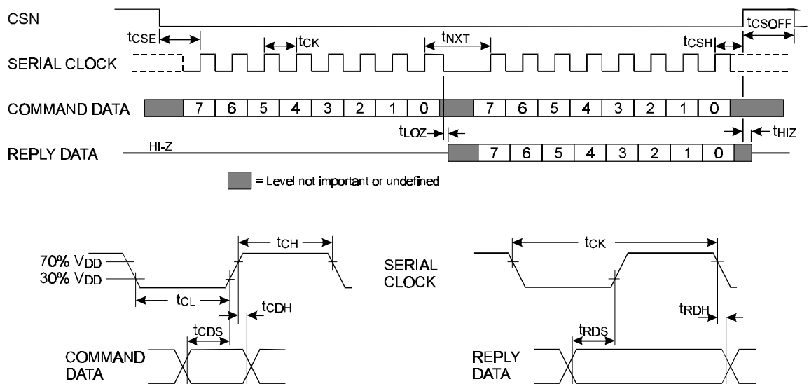
Figure 9 'C-BUS' Timing
