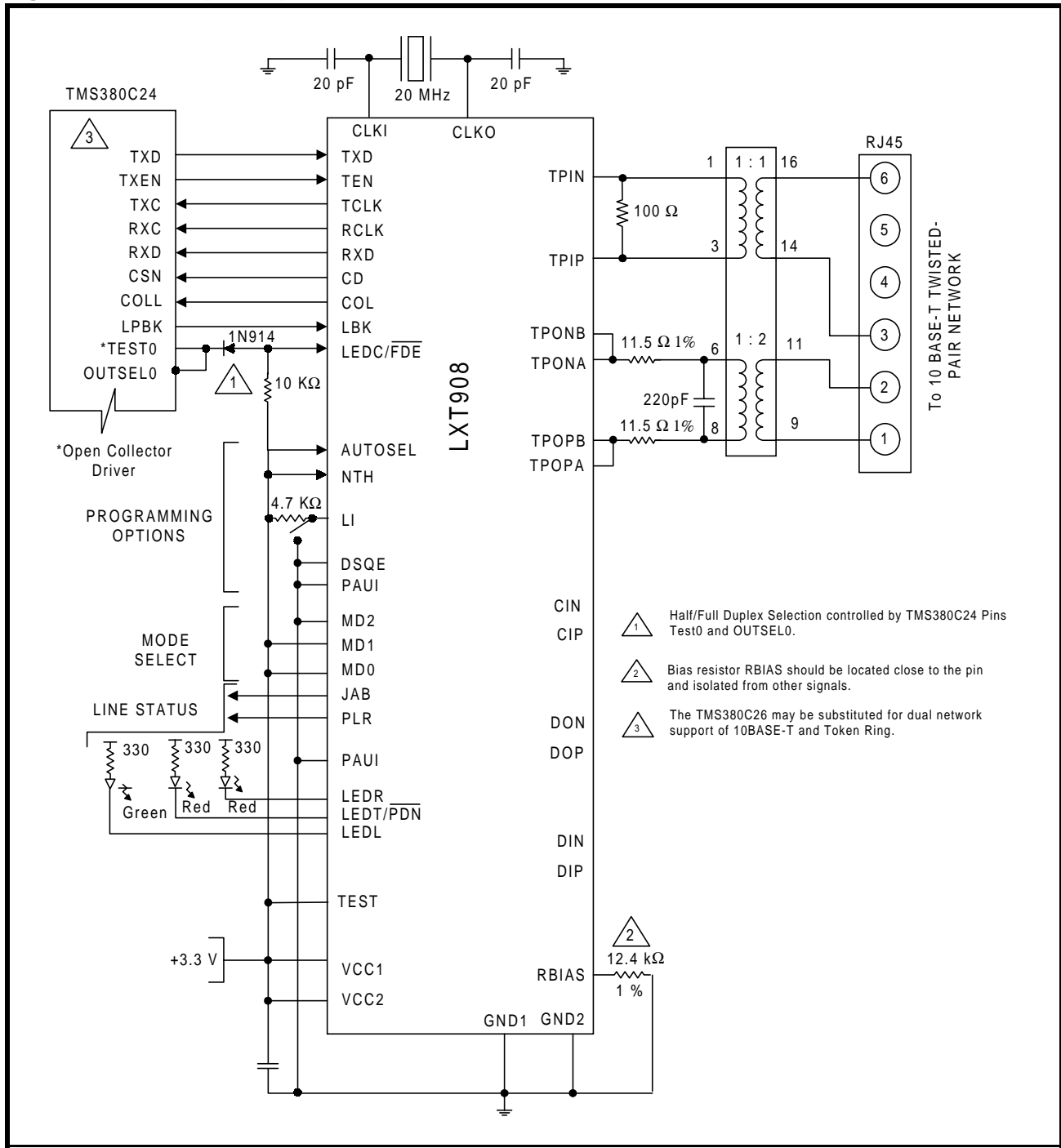
Figure 9: Full-Duplex Operation
