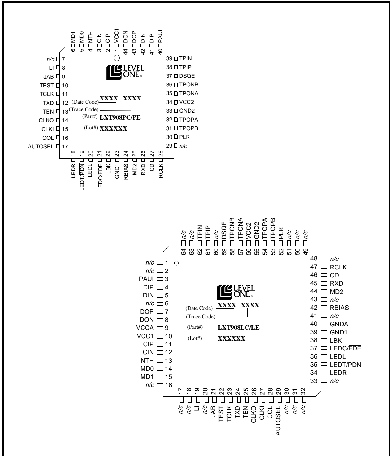
Figure 1: LXT908 Pin Assignments
