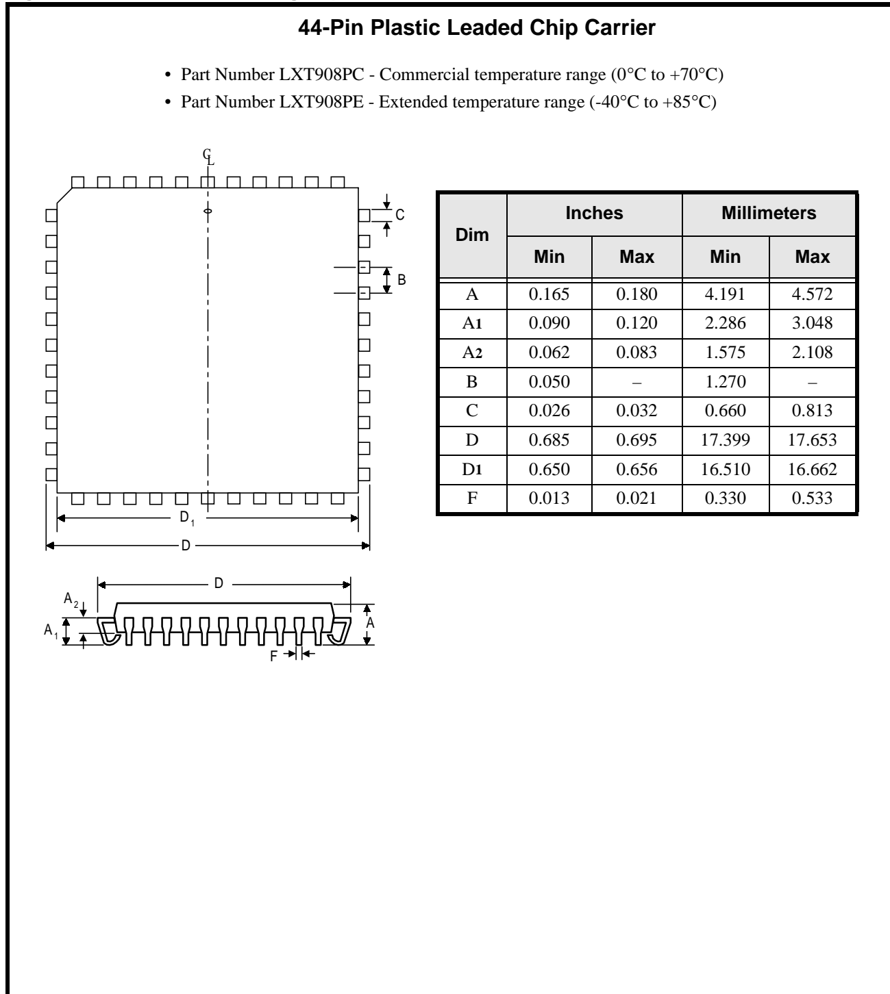
Figure 45: 44-Pin PLCC Package Specifications
